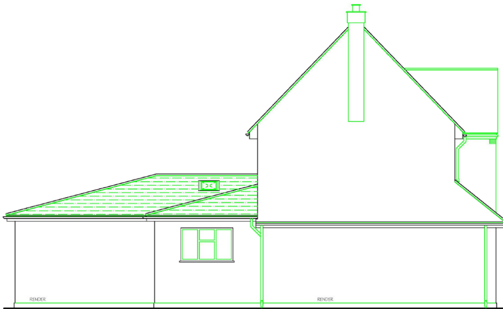
PROPOSED L-SIDE ELEVATION
