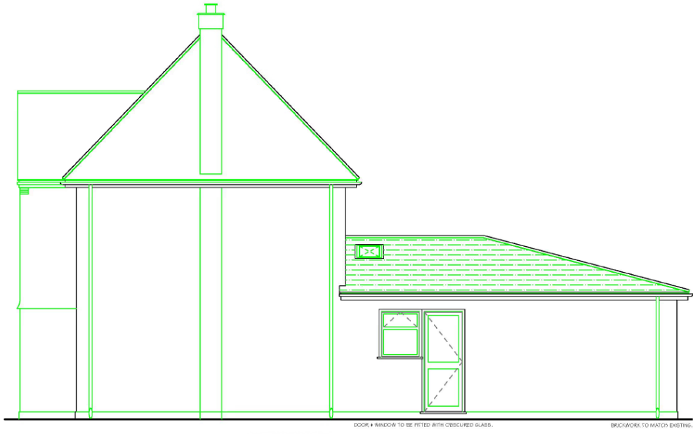
PROPOSED R-SIDE ELEVATION
